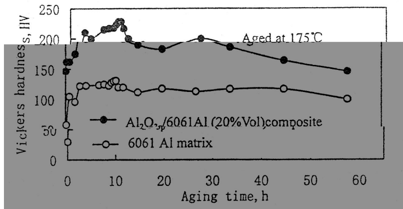
3-3 Al_2O_3/6061A (20% Vol)
